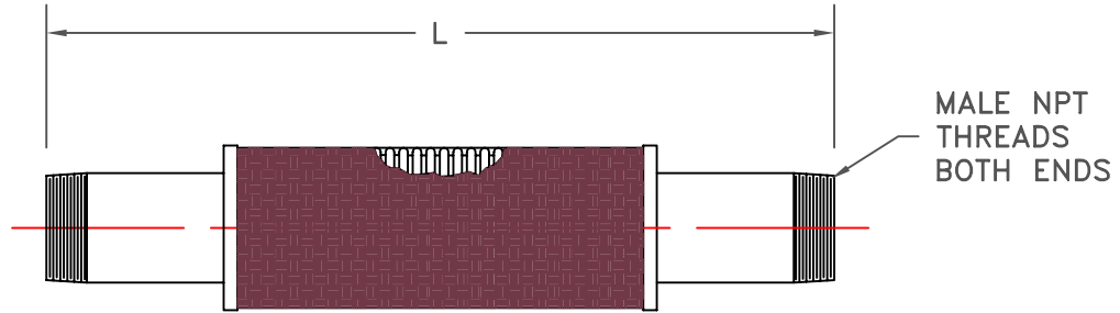
KINFLEX BFMC-MTE
